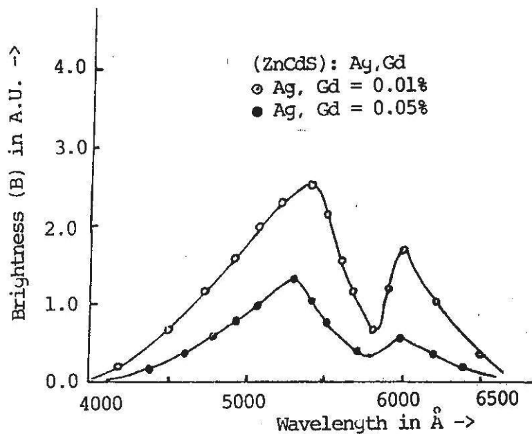
Fig. 3. PL spectra of (ZnCdS): Ag, Gd phosphor.
